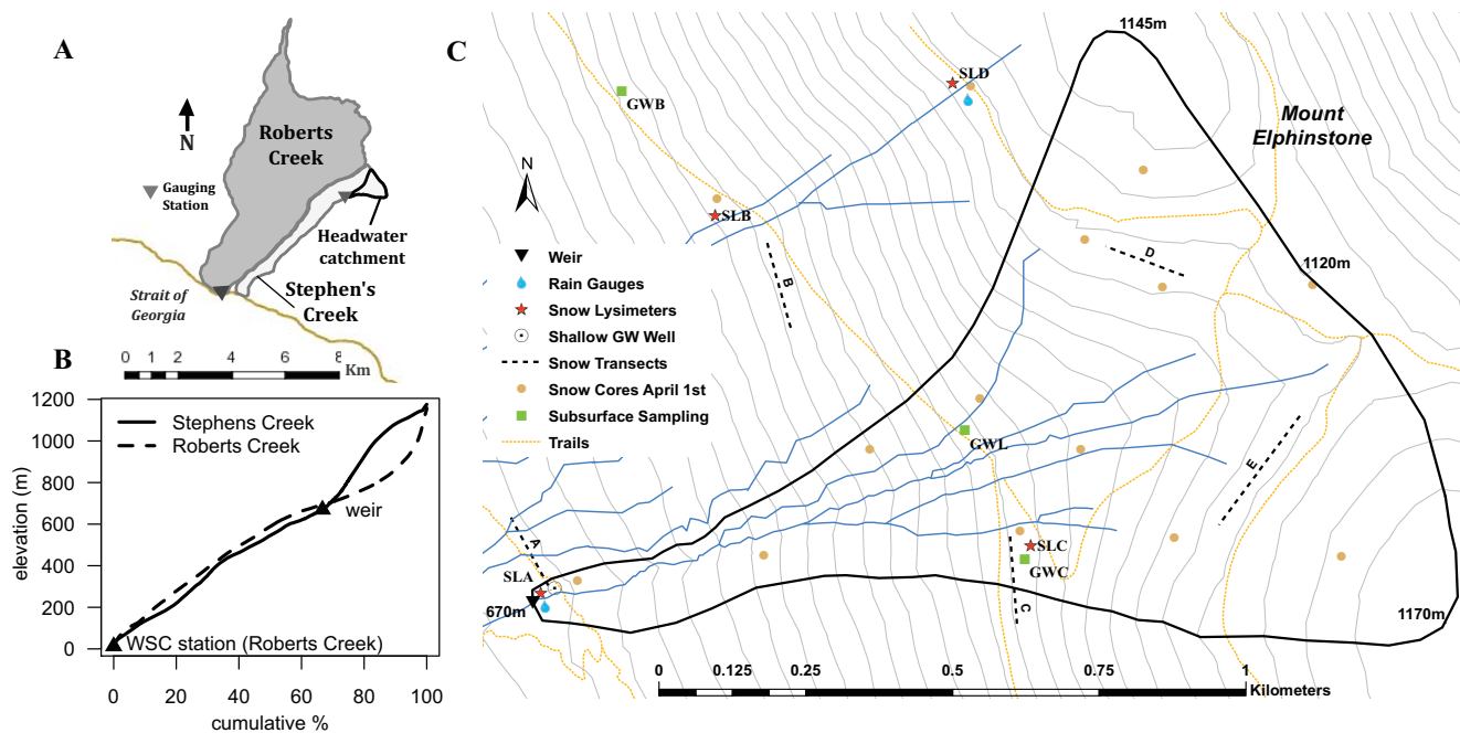
Figure 1. (a) Localization of the research area, (b) hypsometric curves of Roberts Creek and Stephen's Creek watersheds, and (c) instrumentation of the catchment area, Stephen's Creek headwater
