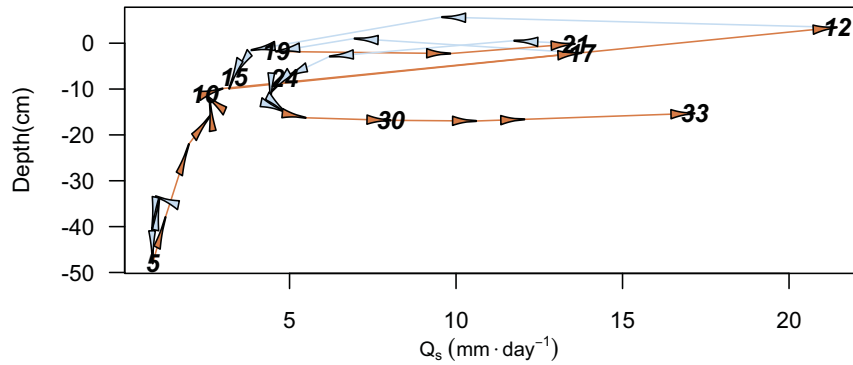
Figure 2. Stephen's Creek discharge at the weir plotted against shallow groundwater-level from April 1 st to May 3 rd 2009 (day 1 to 33, some are numbered). The rising limb is coloured brown and the falling limb is light blue.
