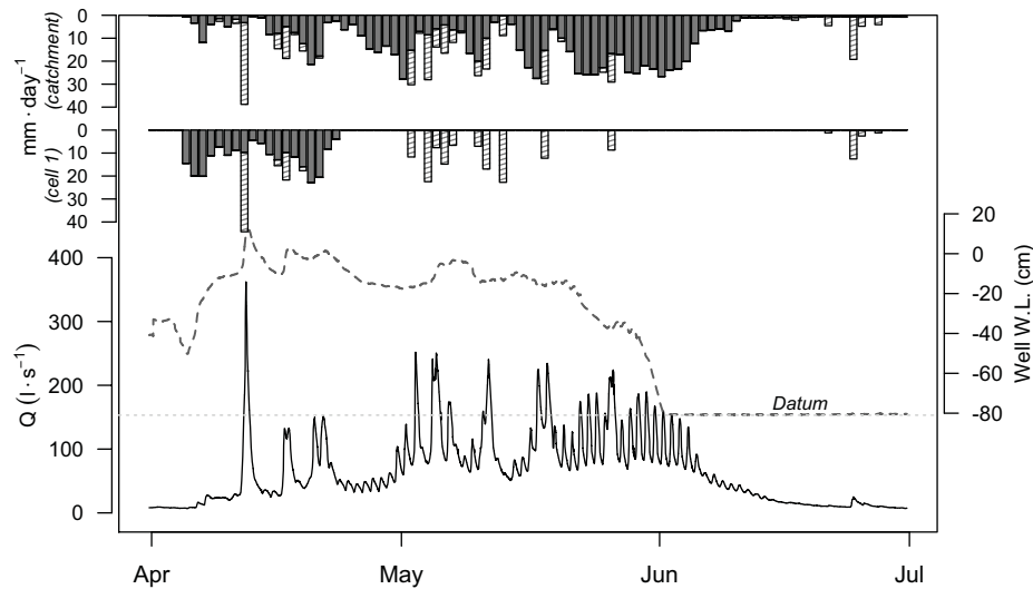
Figure 3. Instantaneous discharges for Stephen's Creek at the weir (solid line), piezometer water-level fluctuations (dashed line). The upper bar plot represents the area-weighted average snowpack drainage-output for the whole catchment (solid bars are snowmelt as modelled by YAM and gradient bars are throughfall) while the lower bar plot shows the modelling-cell where the piezometer is located.
