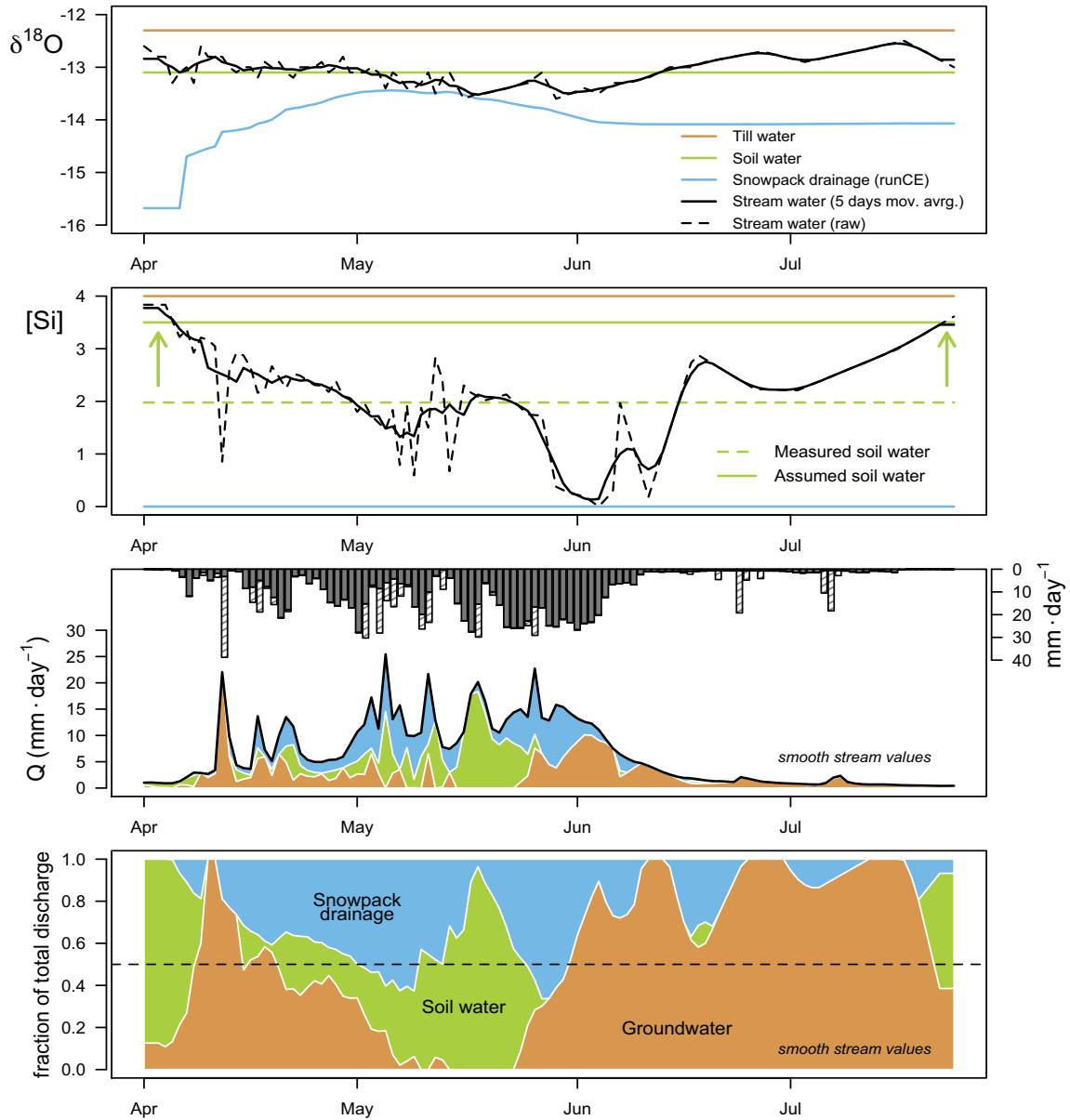
Figure 5. Three-component hydrograph separation using an assumed silicon concentration to define the soil water component. Upper two graphs show component and stream concentrations for both tracers; the 2 nd lower graph shows the hydrograph separation and the most lower graph shows the corrected fraction of groundwater, soil water and snowpack water in the streamflow for smothered stream concentrations
