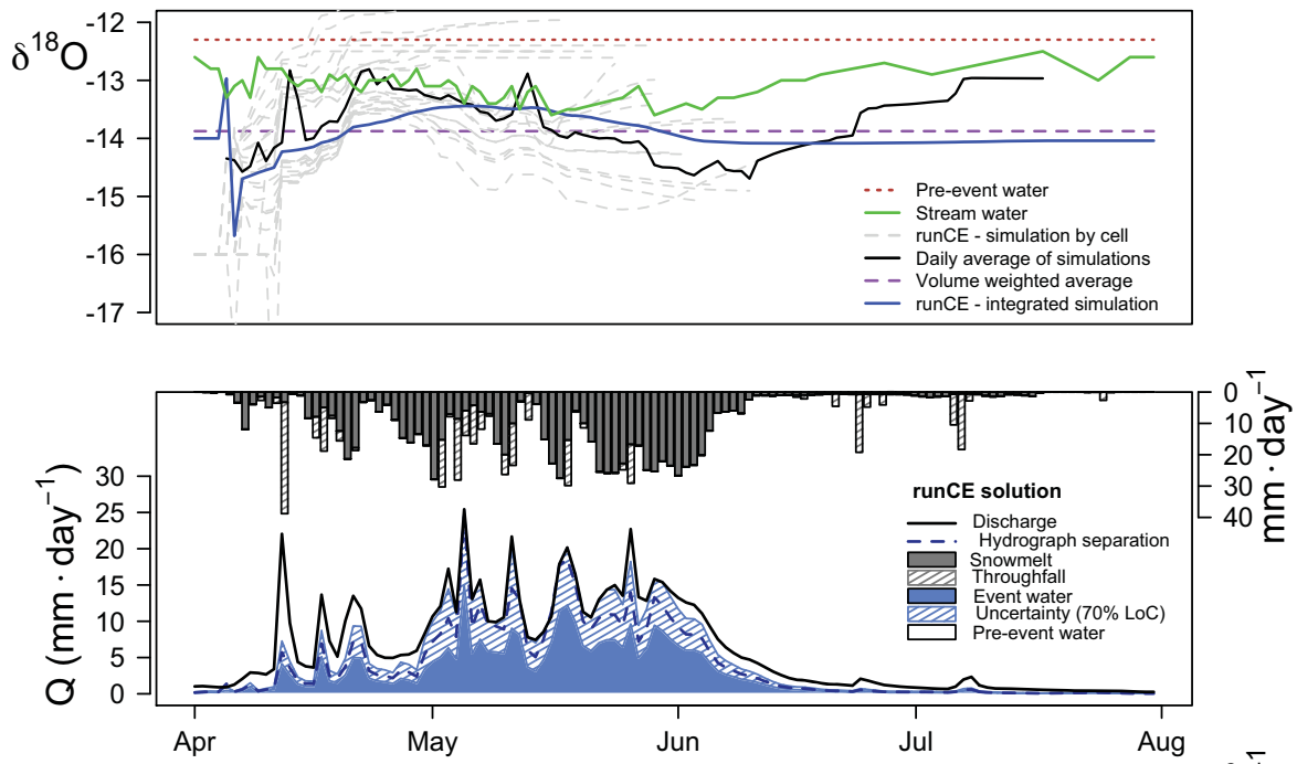
Figure 4. Two-component hydrograph separation results. Upper graph: isotopic signature of components and output from the runCE simulation (event water). Lower graph: hydrograph separation using the runCE method.
