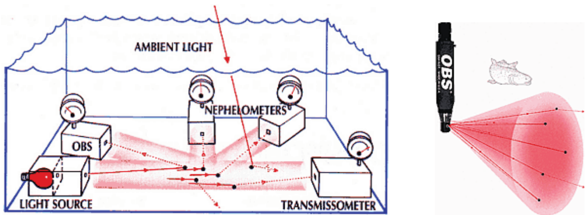
Figure 1. The sketch on the left shows how various devices detect a light source created by a red light bulb. The sketch on the right illustrates the angle in which the OBS-3 detects the scattered light.
