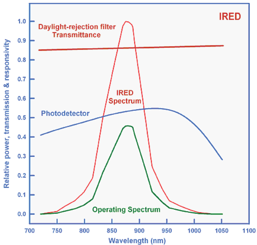
Figure 2. Graph shows the relative power, transmission, and responsivity of a IRED diode. The bandwidth of the IRED is ~40 times wider than laser diodes.
