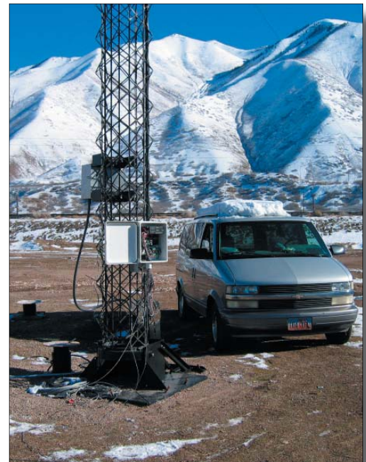
This wind assessment site uses a Campbell Scientific data acquisition system to collect data from an IsoTruss tower and sensors.
