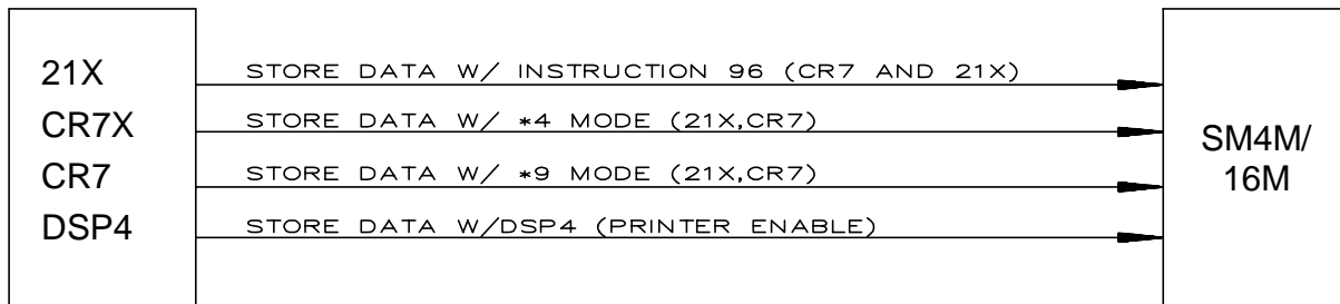
FIGURE 1-3. Pin-Enable Operations
