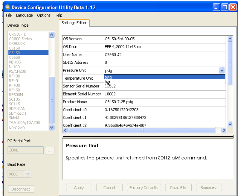
FIGURE 3-6. Configure Units
