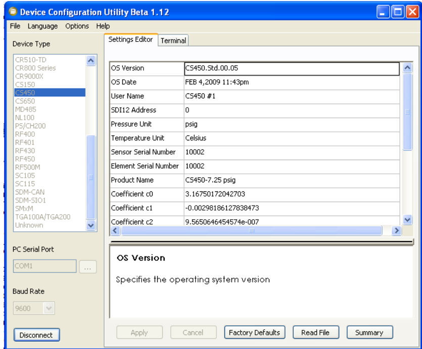
FIGURE 3-5. Connect Screen
