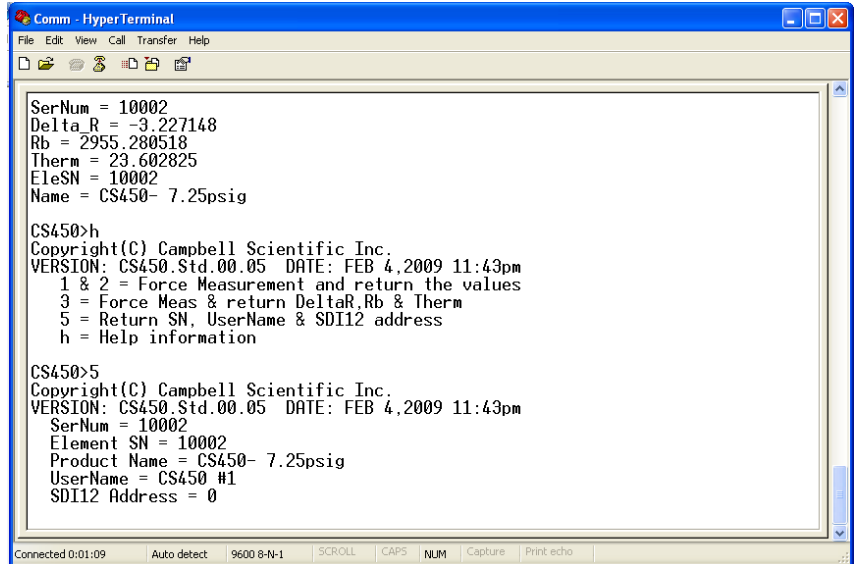
FIGURE 3-3. HyperTerminal
