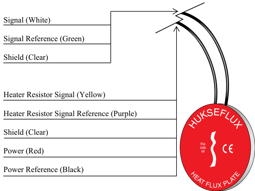
FIGURE 2. HFP01SC Plate
