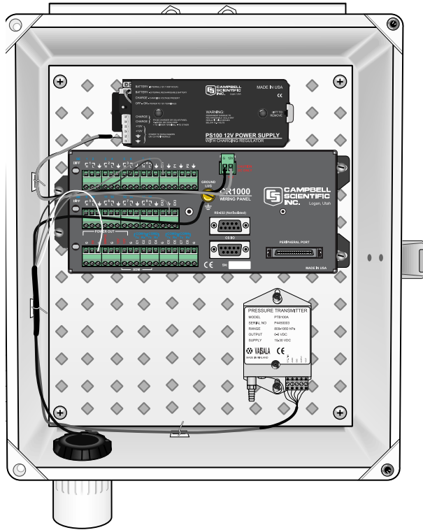
FIGURE 1. CS105 Mounted on the Backplate of an ENC12/14 Enclosure, and Connected to a CR1000 Datalogger
