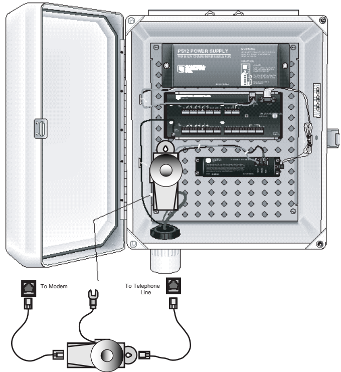
An ENC 12/14 enclosure housing a CR10X, PS12LA power supply, a COM300, an SC12 cable, and surge protector (C1428). Sensor cabling and solar panel not shown
