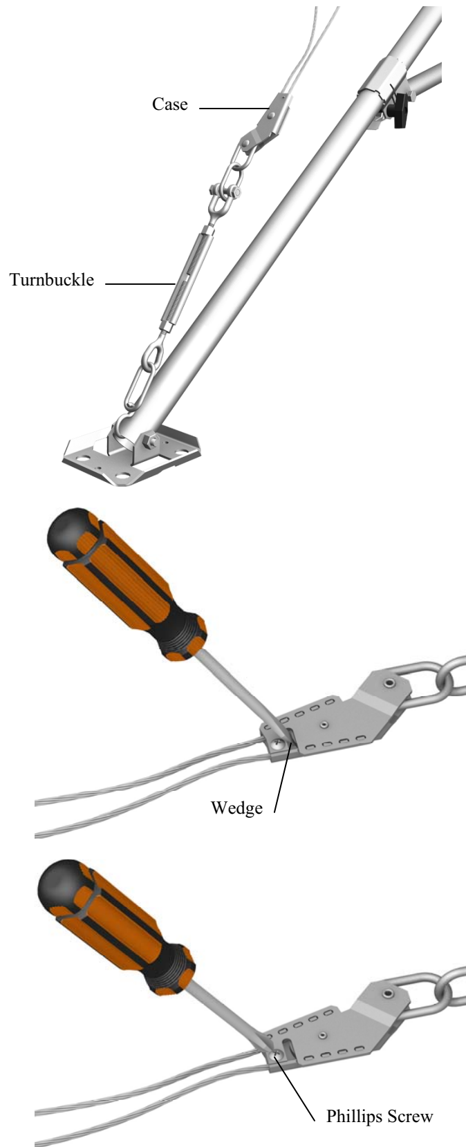
FIGURE 5-6. Leg Attachment
