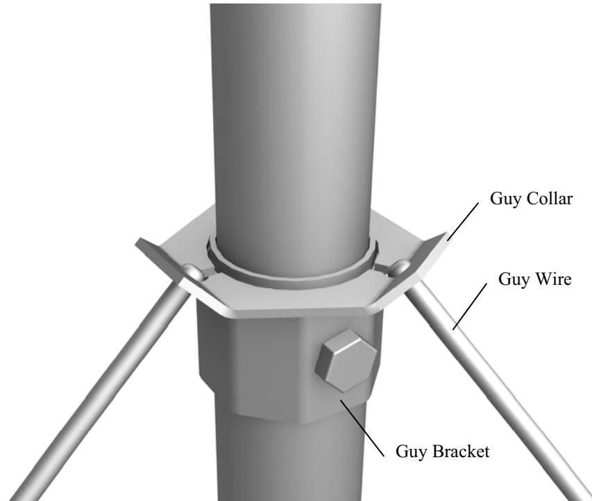
FIGURE 5-5. Guy Collar
