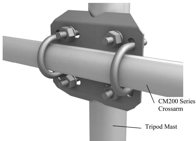
FIGURE 5-10. CM204 Crossarm
