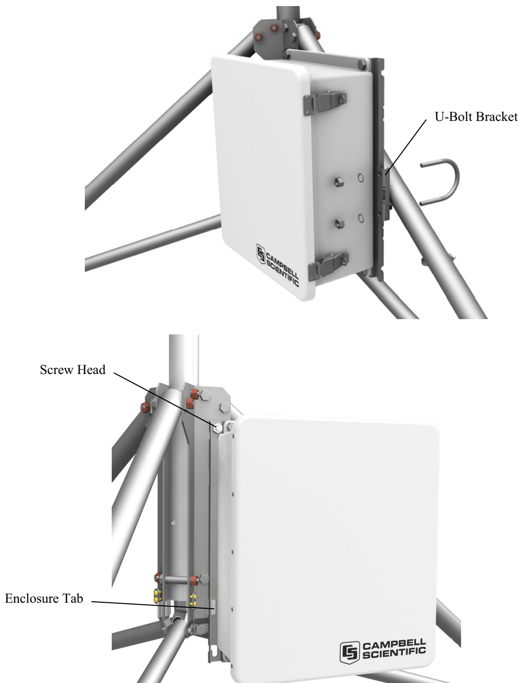
FIGURE 5-12. Enclosure with the -LM Bracket
