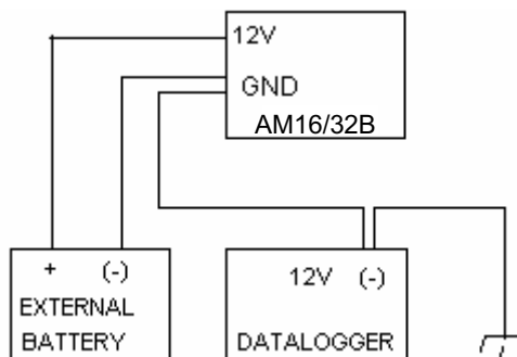
FIGURE 5. Power and Ground Connections for External Power Supply
