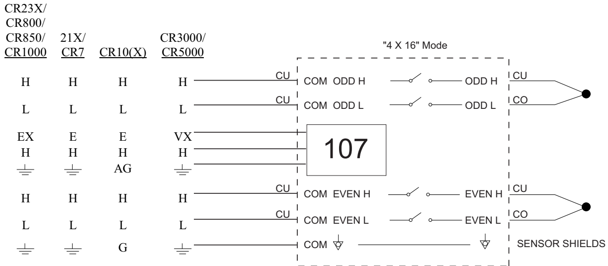
FIGURE 18. Differential Thermocouple Measurement with Reference Junction at the Datalogger
