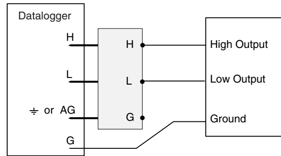
CURS100-to-Sensor Hookup
