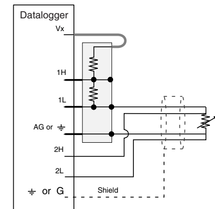
Module-to-Sensor Hookup
