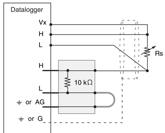
4WHB10K-to-Sensor Hookup
