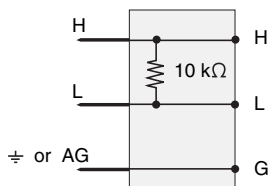
4WHB10K Schematic
