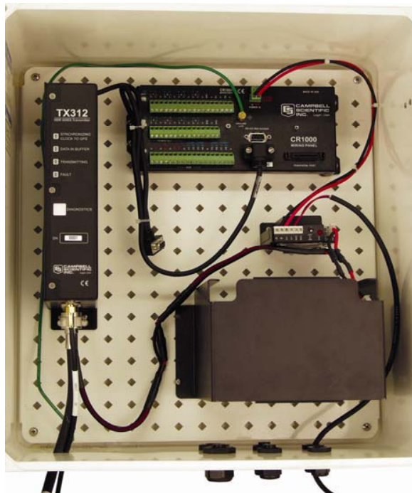
FIGURE 3-3. DCP Enclosure
