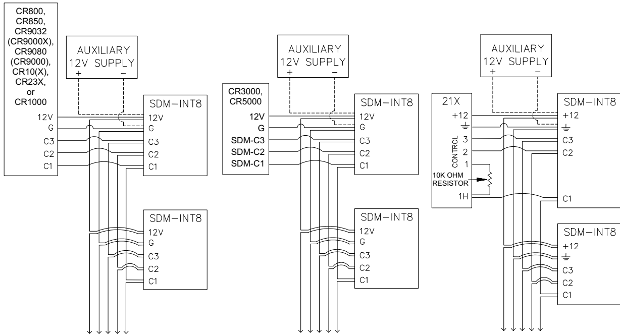
FIGURE 3. Wiring Diagram
