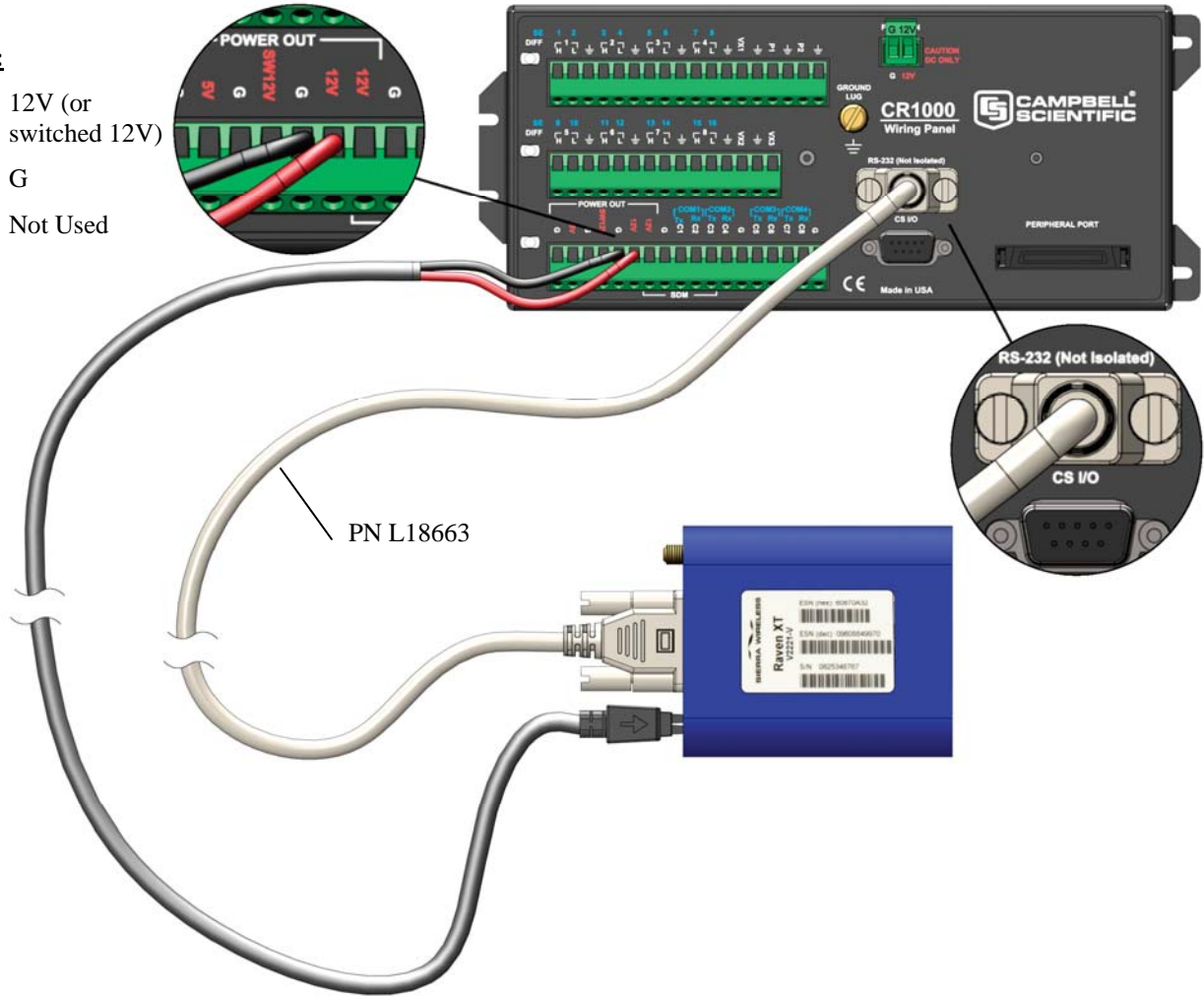
PN L18663 Null Modem Cable—connects the modem to the CR23X, CR3000, CR800, CR2XX, CR1000 or CR5000 RS-232 port (not compatible with the 21X, CR510, CR10X, or CR7 dataloggers).
