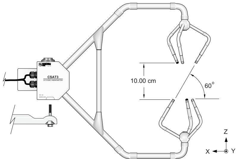
FIGURE 1. CSAT3 Coordinate System and Captive Mounting Hardware (s/n 0631 to current)
