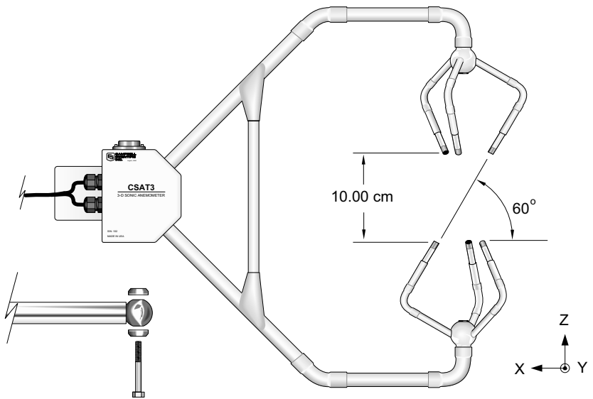
FIGURE 3. CSAT3 Coordinate System and Original Noncaptive Mounting Hardware (s/n 0107 to 0630)
