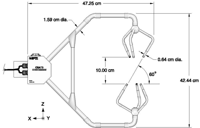
Anemometer Head
