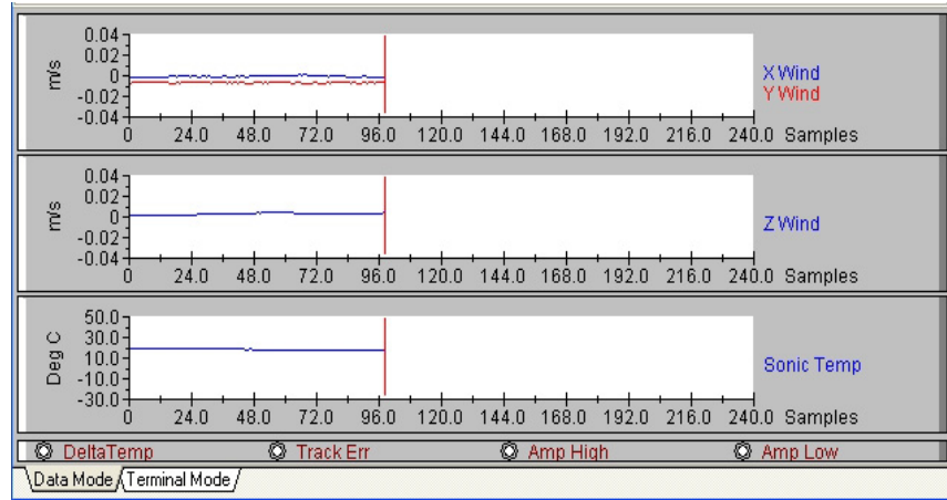
FIGURE 10. Wind Data from CSAT3 s/n 315; Wind Offsets within Specifications at 19°C.
