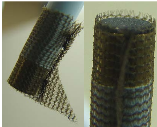
FIGURE 6. Proper Location of the Top (p/n 17388) and Bottom (p/n 17389) Wicks
