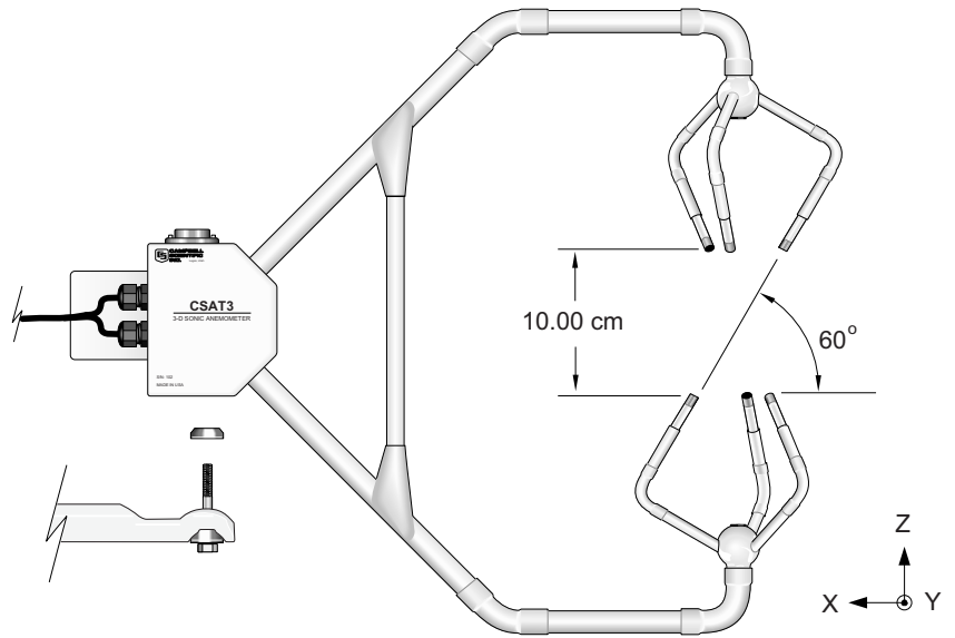
FIGURE 2. CSAT3 Coordinate System, and Captive Mounting Hardware and Cup Washer (s/n 0107 to 0630)
