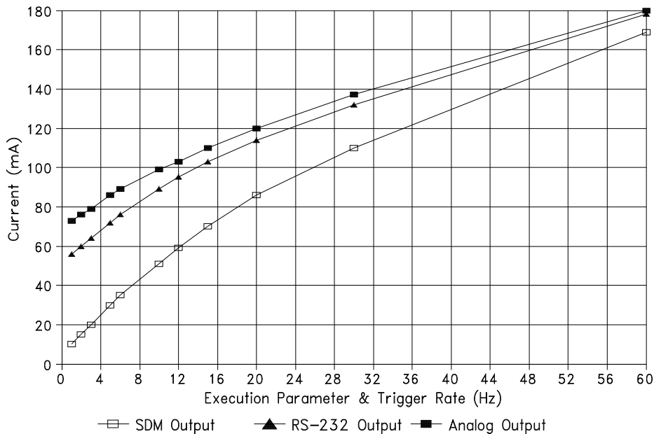
FIGURE 4. Typical Average CSAT3 Current Drain at +12 VDC
